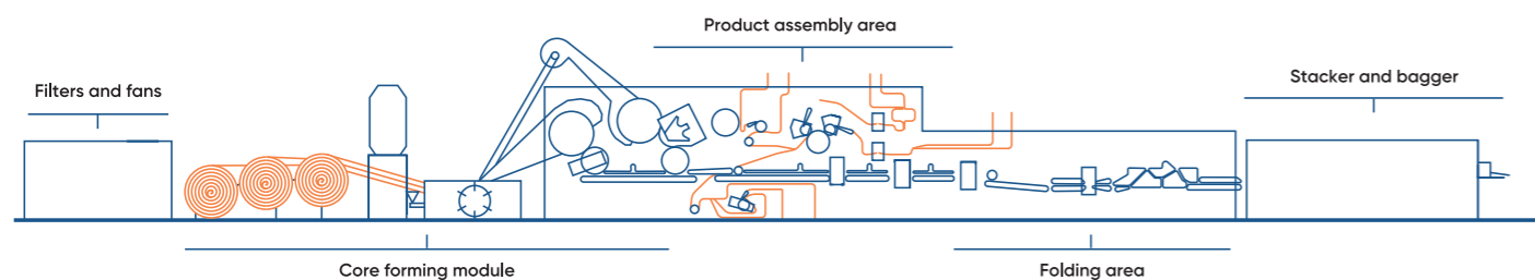
Easy maintenance mezzanine
