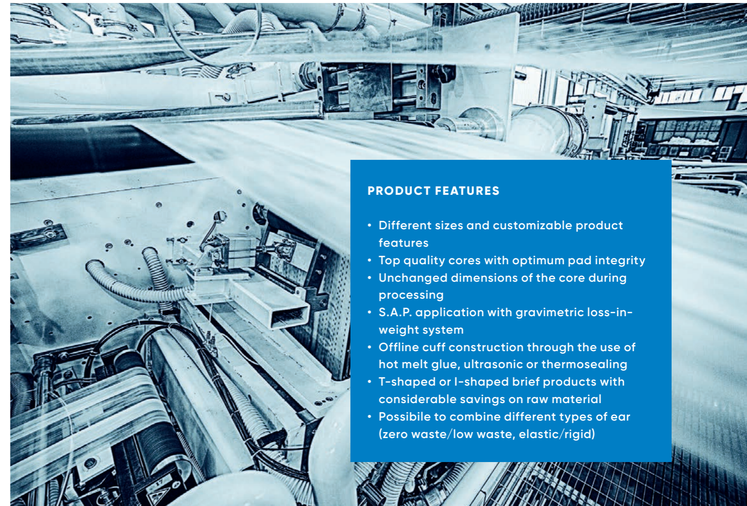
Web entry in-line
